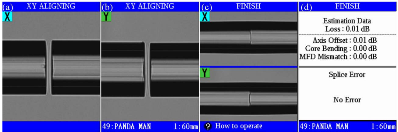
Figure 2. Images of the PM fibers spliced with rotation of their birefringence axes by 90^\circ relative to each other inside the ring fiber cavity (as marked by a cross in Fig. 1) before [(a) and (b)] and after splicing [(c) and (d)].
